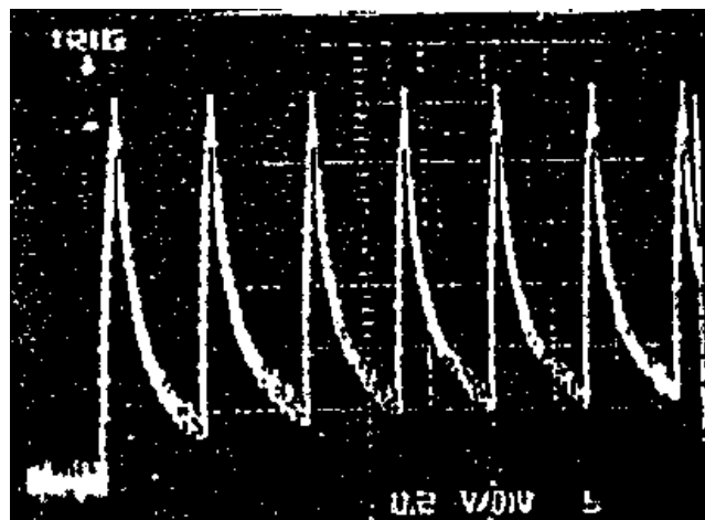
FIGURE 5. Voltage Fluctuation
