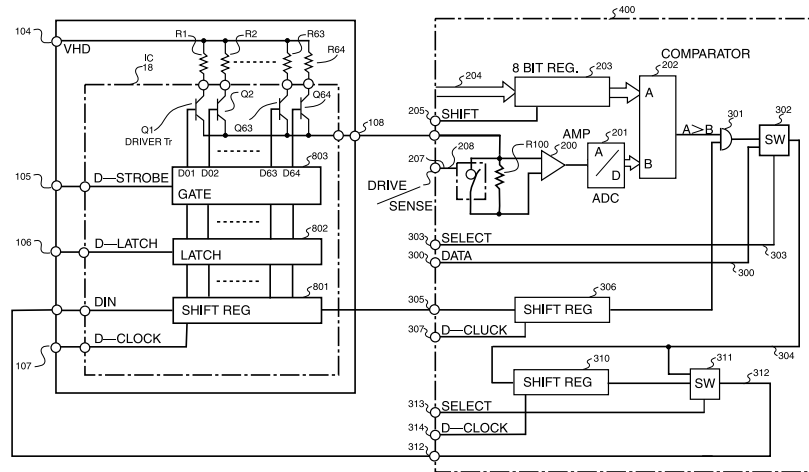
FIGURE 4. Head Control Circuit Structure
