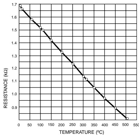
FIGURE 2. Thermistor Characteristics
