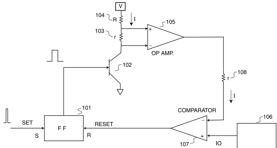
FIGURE 3. Temperature Control Principle
