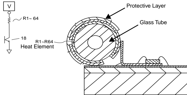
FIGURE 1. Print Head Structure
